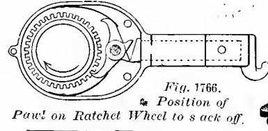
THE HINCKLEY BRAKE SLACK ADJUSTER EQUIPMENT D.
